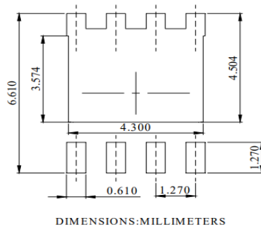
DIMENSIONS: MILLIMETERS
