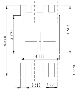
DIMENSIONS:MILLIMETERS
