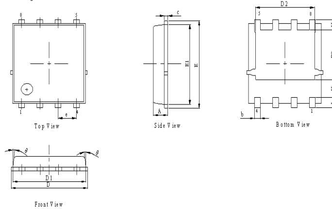
Package Outline
