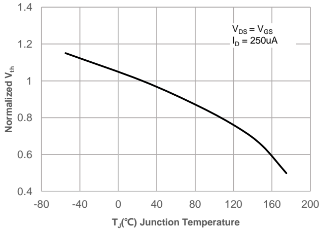
Figure 13: Normalized Threshold Voltage vs. Junction Temperature
