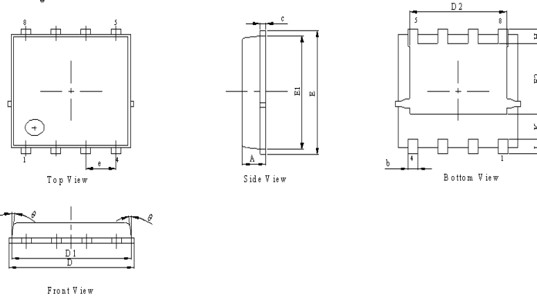
Package Outline
