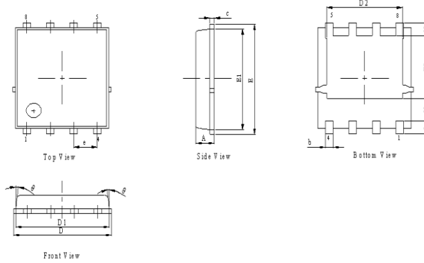
Package Outline
