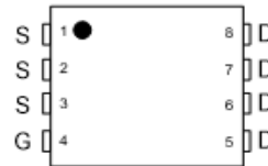
Pin Assignment
