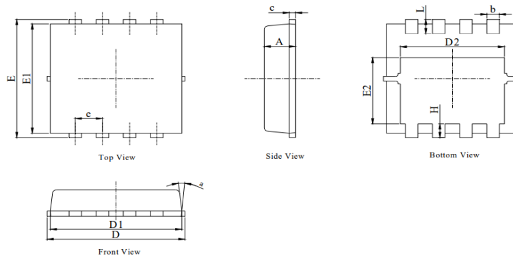
Package Outline
