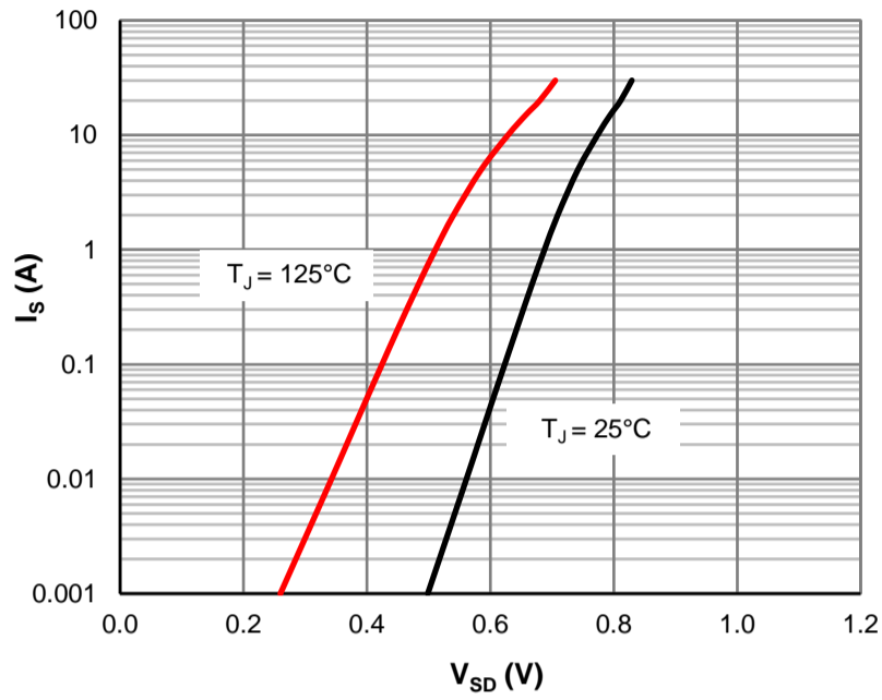
Figure 7: Body-Diode Characteristics
