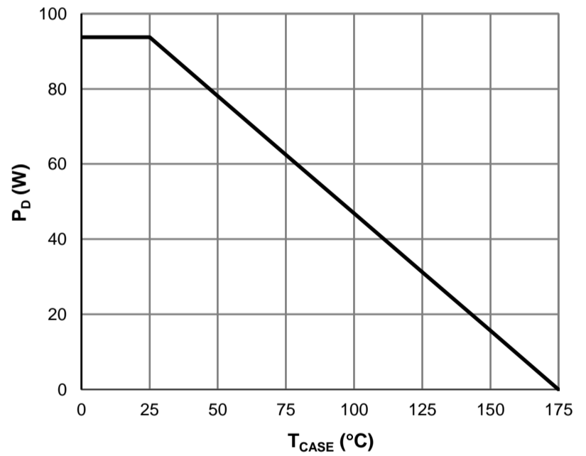
Figure 10: Power De-rating
