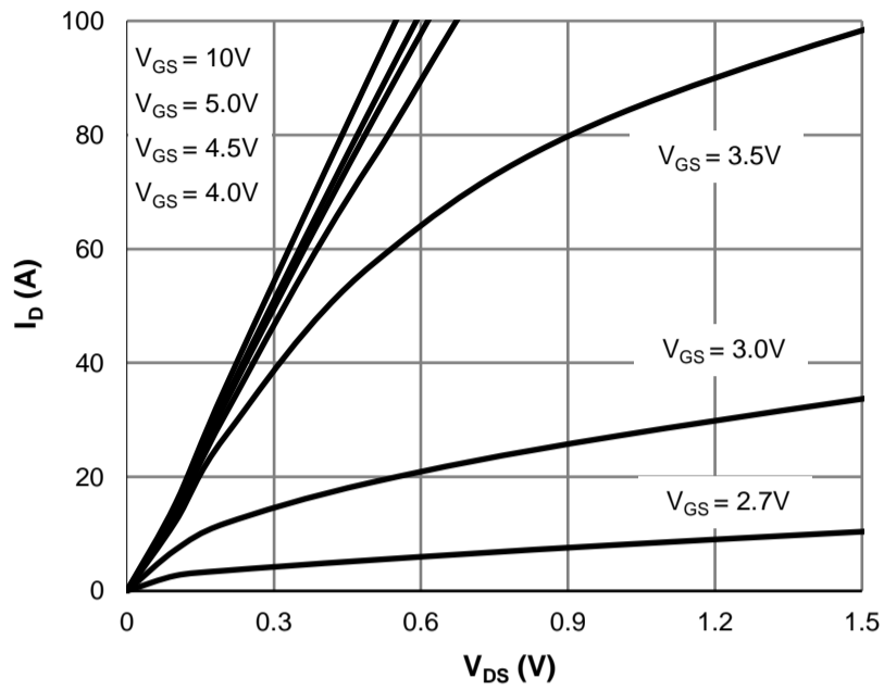
Figure 1: Saturation Characteristics
