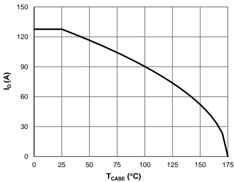
Figure 9: Current De-rating
