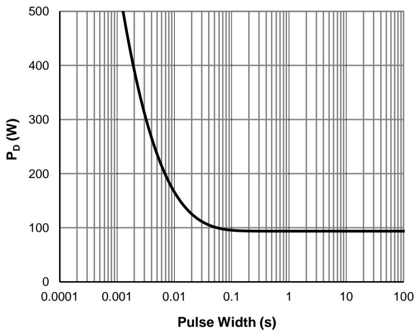
Figure 11: Single Pulse Power Rating, Junction-to-Case
