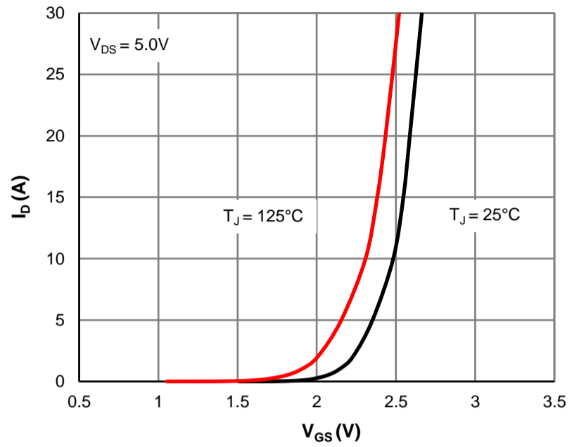
Figure 2: Transfer Characteristics
