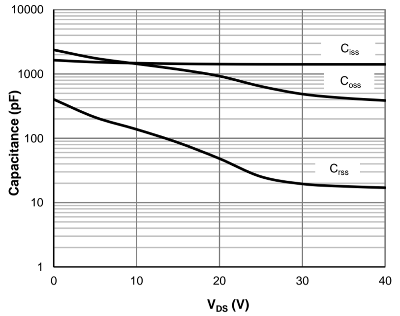
Figure 8: Capacitance Characteristics
