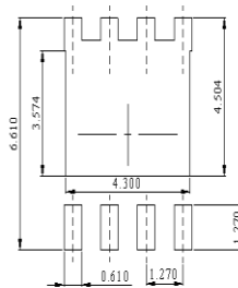
DIMENSIONS: MILLIMETERS
