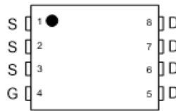
Pin Assignment
