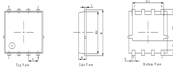
Package Outline
