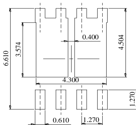
DIMENSIONS: MILLIMETERS
