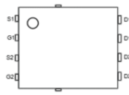
Pin Assignment
