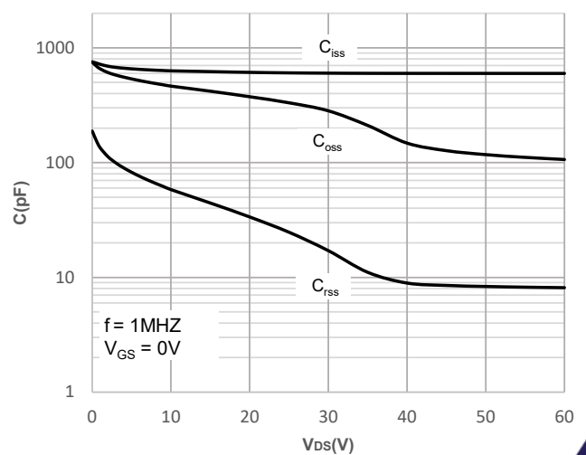
Figure 10: Capacitance Characteristics
