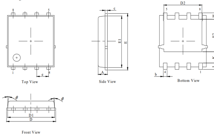
Package Outline
