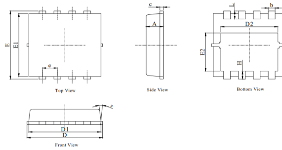
Package Outline
