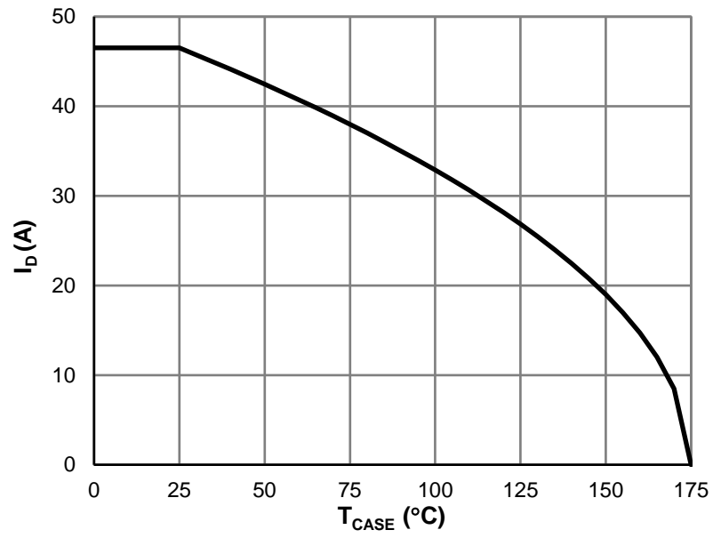
Figure 7: Current De-rating
