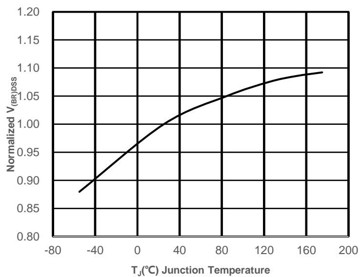
Figure 12: Normalized Breakdown voltage vs. Junction Temperature
