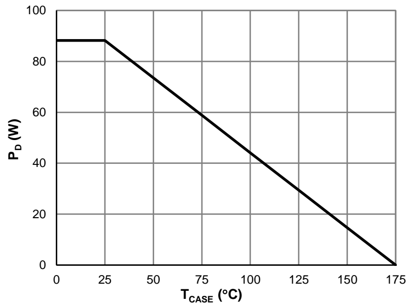
Figure 8: Power De-rating
