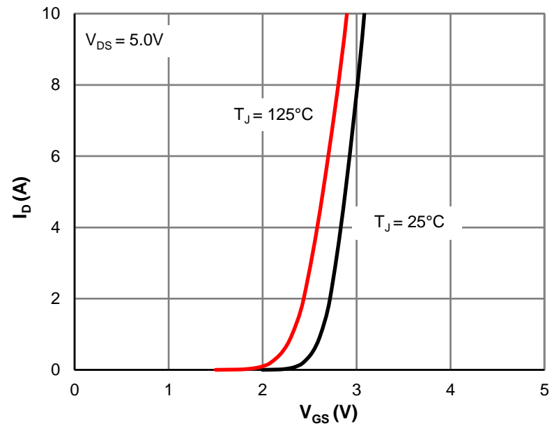
Figure 2: Transfer Characteristics
