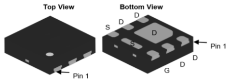
DFN2020-6L
