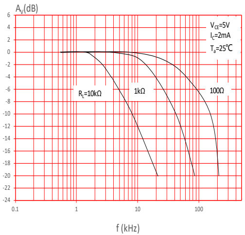
FIG.10: Frequency Response
