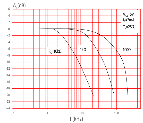
FIG.10: Frequency Response
