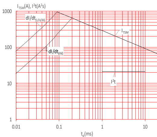
FIG.5: Non-repetitive surge peak on-state current for a sinusoidal pulse with width t_p < 20ms , and corresponding value of I^2t (I-II-III: di/dt < 50A/\mu s ; IV: di/dt < 20A/\mu s )
