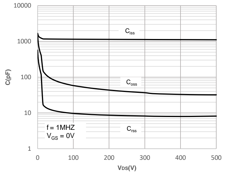
Figure 6: Capacitance Characteristics
