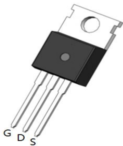
TO-220C-3L Top View
