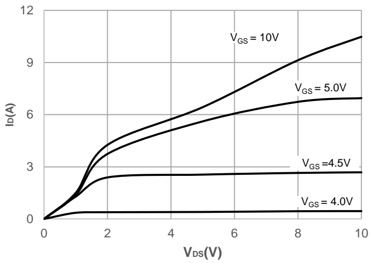
Figure 1: Output Characteristics
