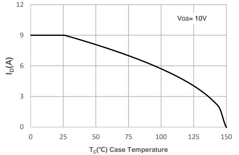
Figure 10: Maximum Continuous Driand Current vs. Case Temperature
