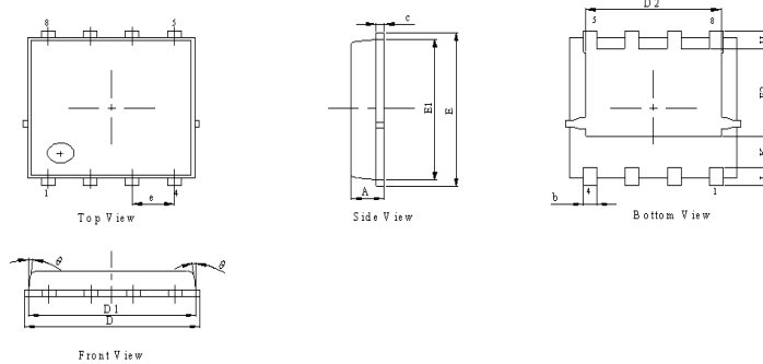
Package Outline
