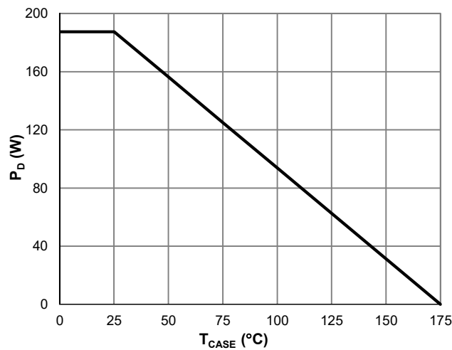
Figure 8: Power De-rating
