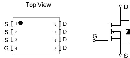
Pin Configuration
