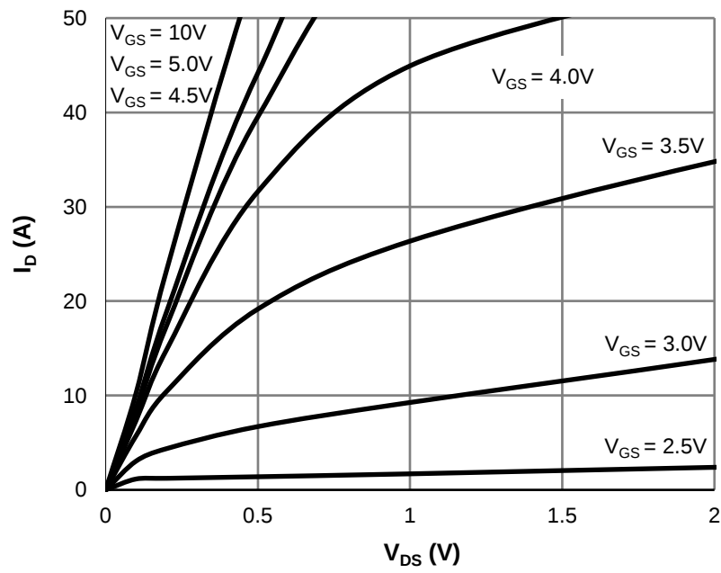
Figure 1: Saturation Characteristics
