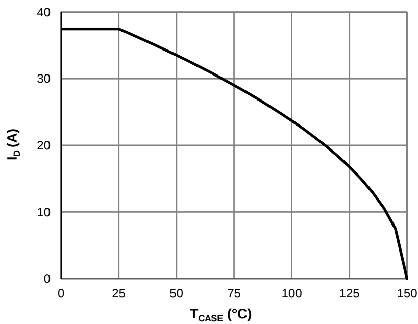
Figure 9: Current De-rating
