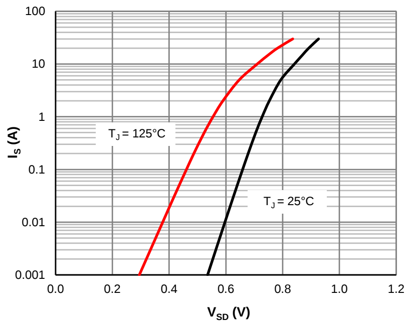
Figure 7: Body-Diode Characteristics
