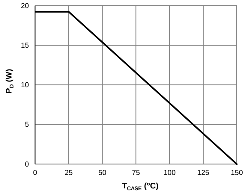
Figure 10: Power De-rating
