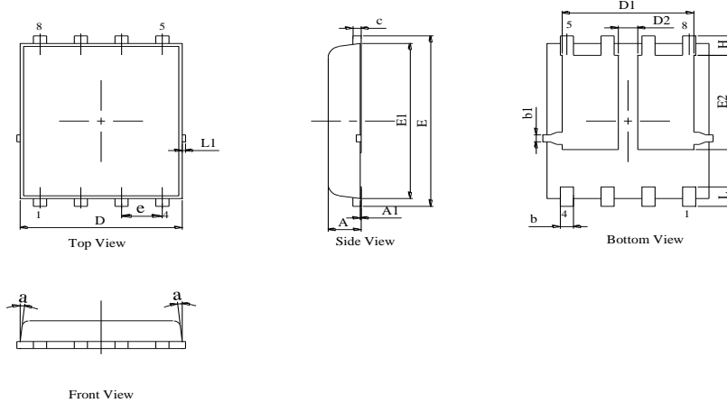
Package Outline
