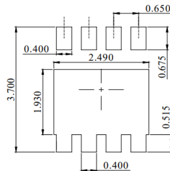
DIMENSIONS:MILLIMETERS
