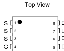
Pin Configuration
