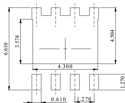
DIMENSIONS: MILLIMETERS
