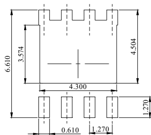
DIMENSIONS:MILLIMETERS
