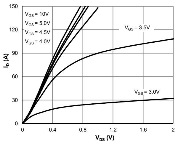
Figure 1: Saturation Characteristics
