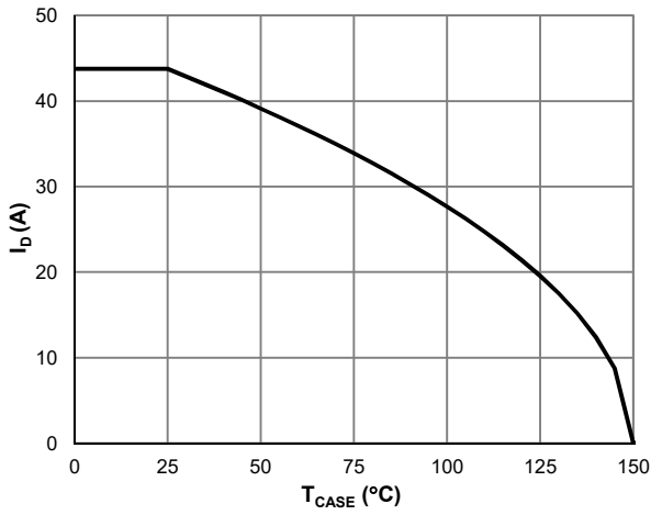
Figure 7: Current De-rating
