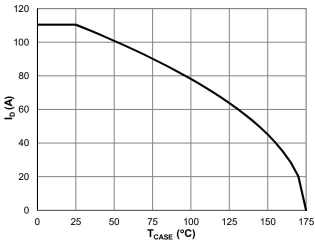
Figure 7: Current De-rating
