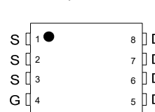
Pin Configuration Top View
