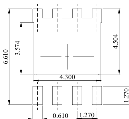
DIMENSIONS: MILLIMETERS
