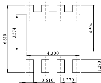
DIMENSIONS: MILLIMETERS
