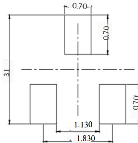
DIMENSIONS:MILLIMETERS
