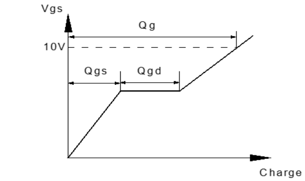
Figure 1: Gate Charge Test Circuit & Waveform
