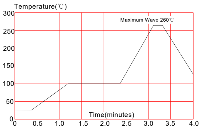
FIG.6: Lead-free profile
