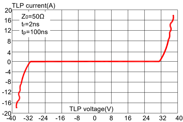
FIG.7: TLP measurement
