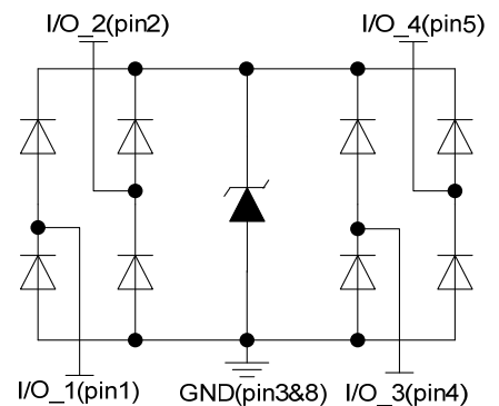
Pin configuration
