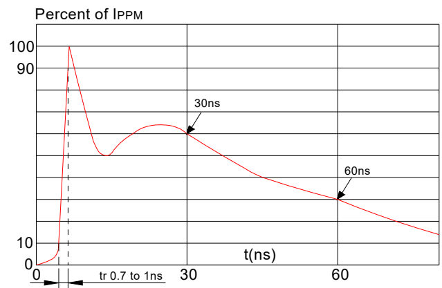
FIG.4: ESD clamping
