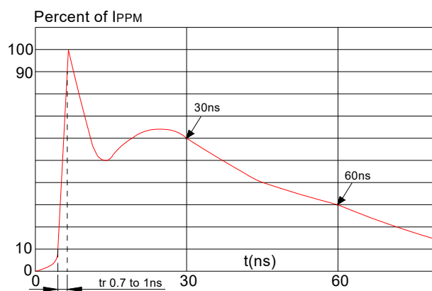
FIG.4: ESD clamping
