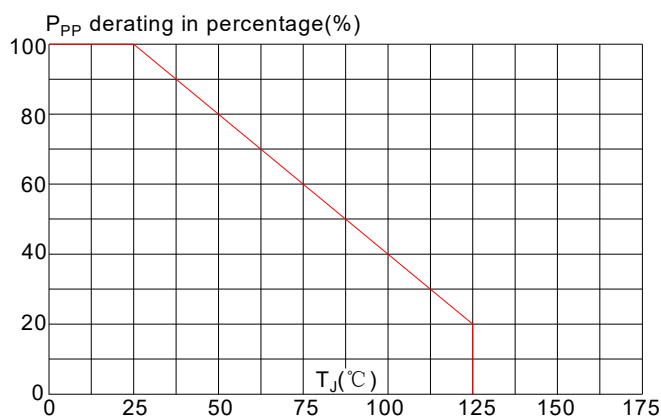
FIG.3: Pulse derating curve
