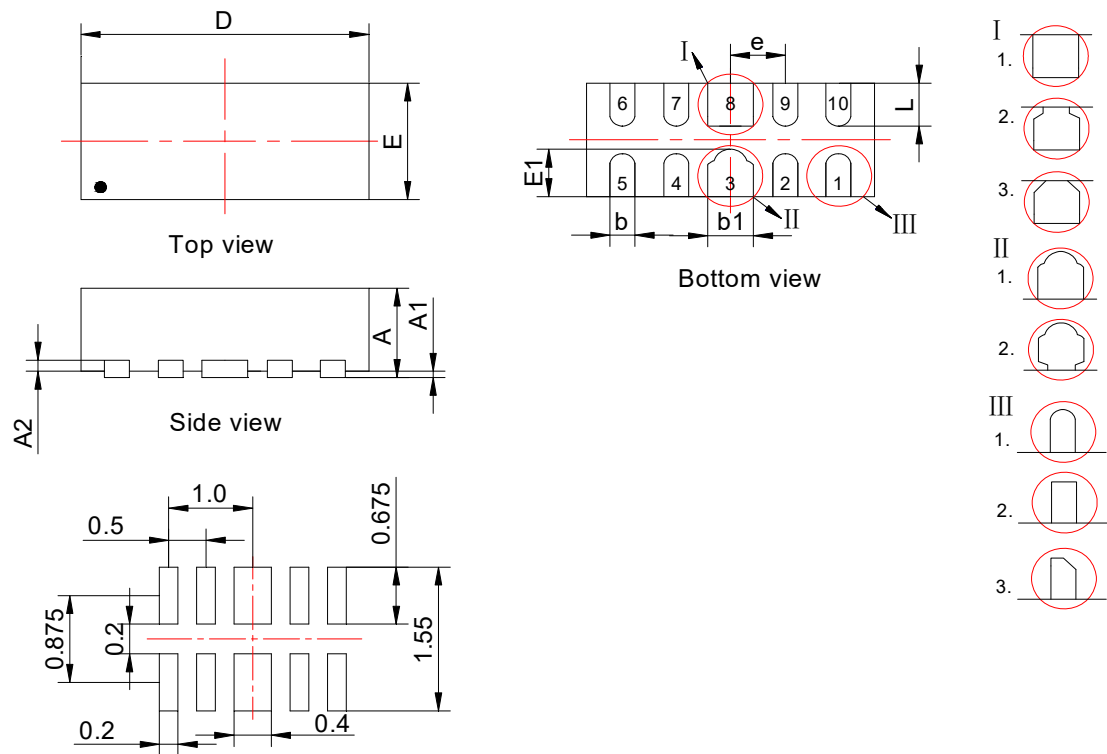
Recommended soldering footprint
