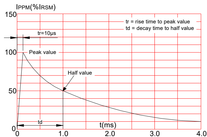
FIG.4: Pulse waveform
