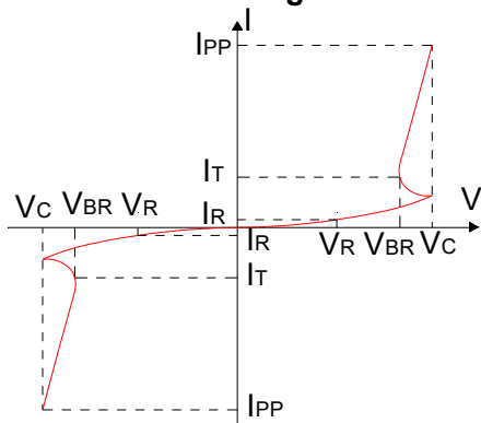
FIG.3:V- I curve characteristics (Bi-directional with negative resistance)
