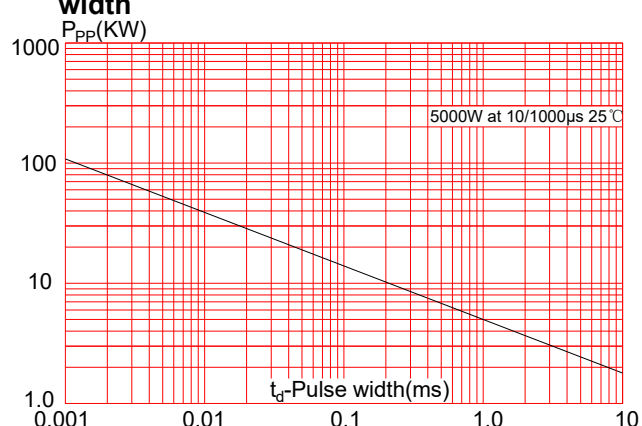
FIG.8: Parameters for test pulse 5a
