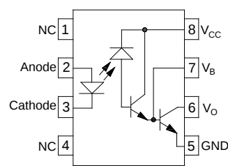
6N138,6N139
