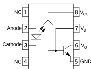
6N135,6N136
