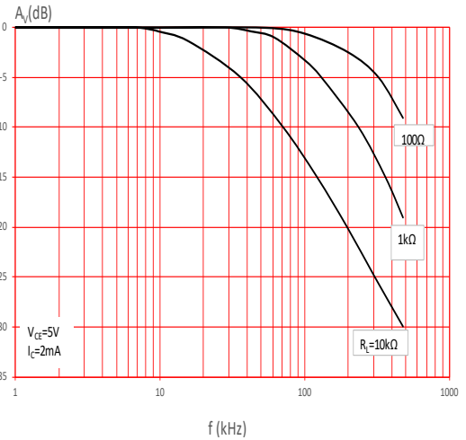
FIG.10: Frequency Response
