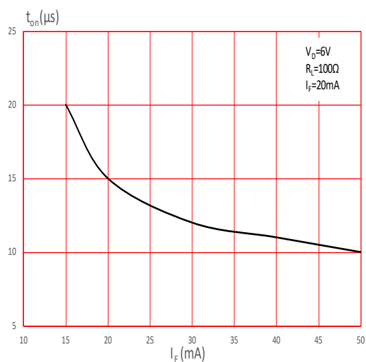
FIG.10: Turn On Time vs. Forward Current
