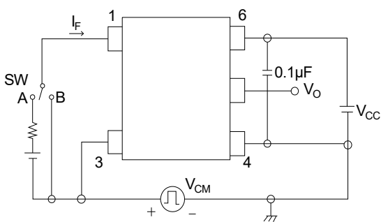
FIG.15: Common-Mode Transient Immunity Test Circuit and Waveform
