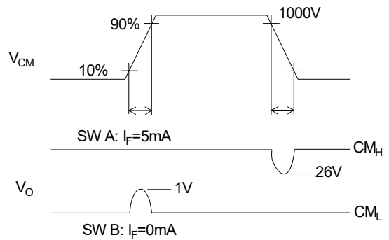
FIG.15: Common-Mode Transient Immunity Test Circuit and Waveform
