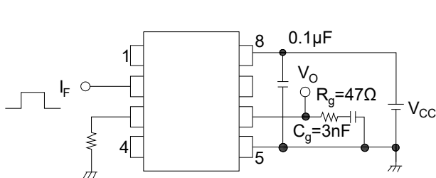
FIG.14: Switching Time Test Circuit and Waveform
