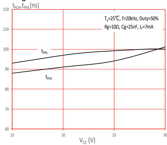
FIG.13: Propagation Delay Time vs. Supply
