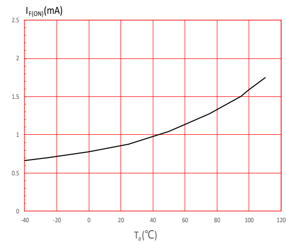
FIG.3: LED Operate Current vs. Ambient Temperature
