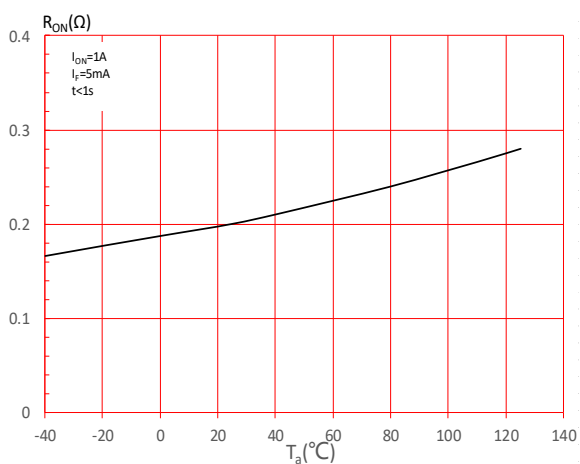
FIG.5: On Resistance vs. Ambient Temperature
