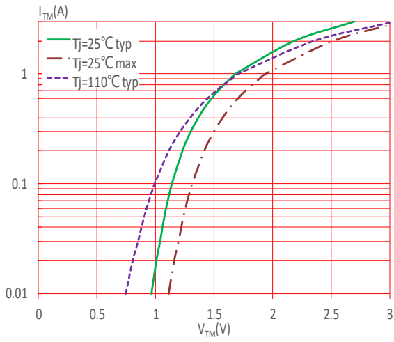
FIG.7: On-state characteristics
